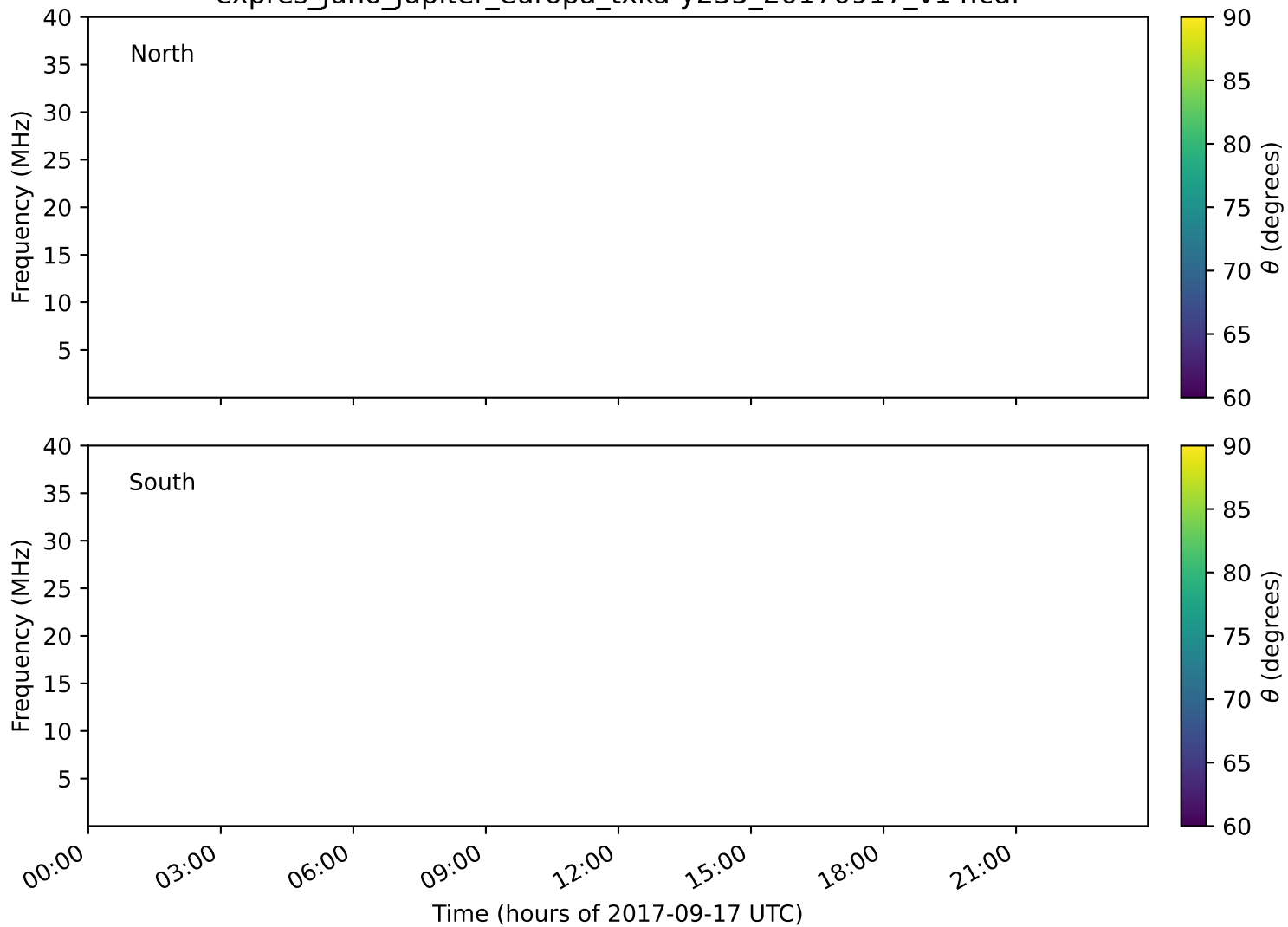
expres_juno_jupiter_europa_txka-y235_20170917_v14.cdf
