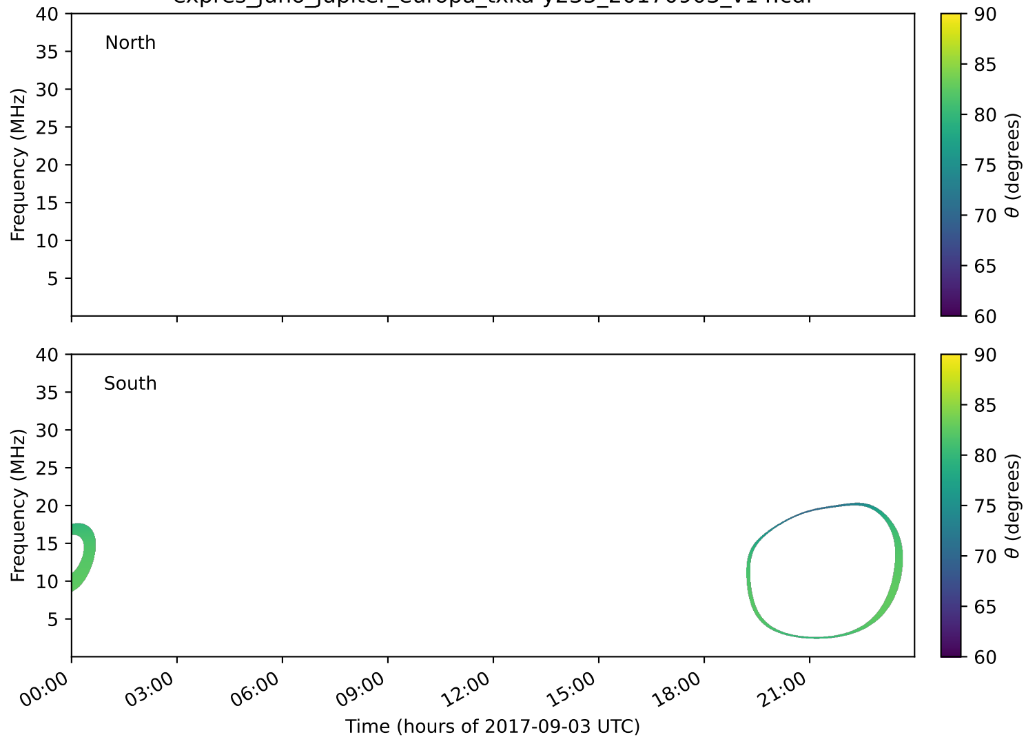
expres_juno_jupiter_europa_txka-y235_20170903_v14.cdf
