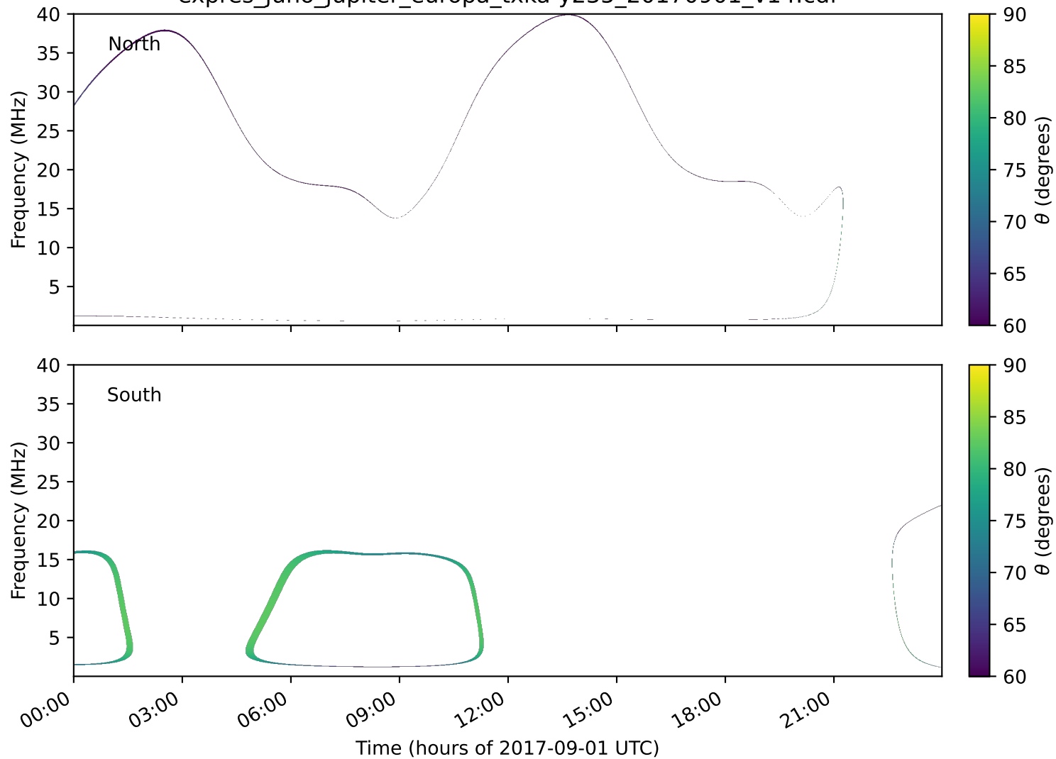
expres_juno_jupiter_europa_txka-y235_20170901_v14.cdf
