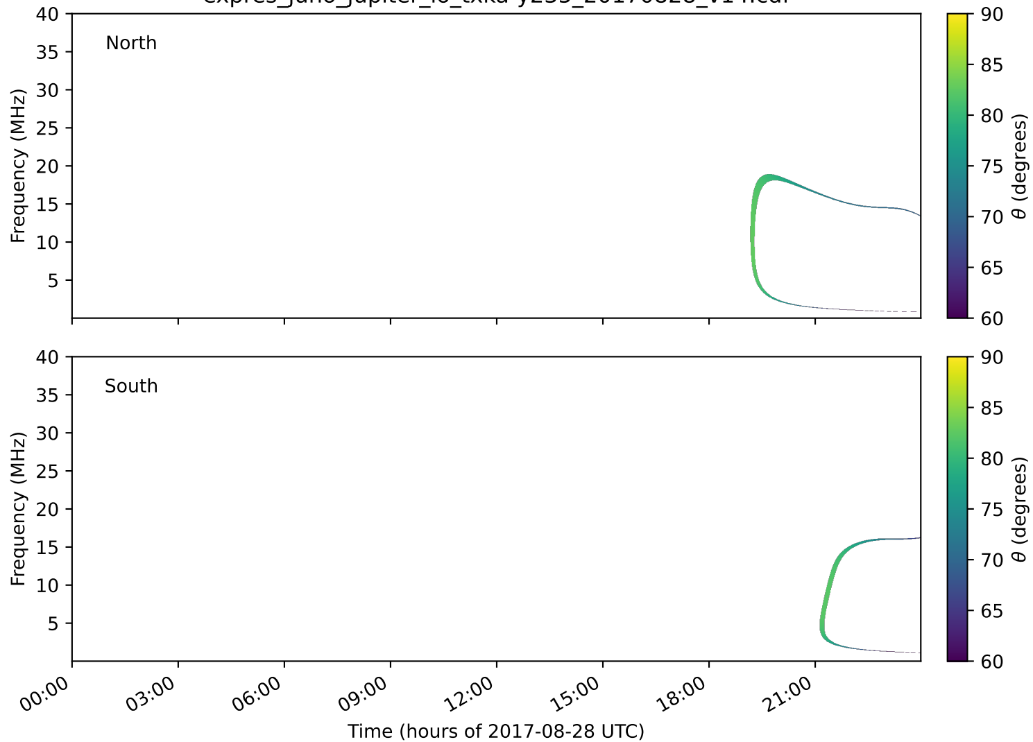
expres_juno_jupiter_io_txka-y235_20170828_v14.cdf
