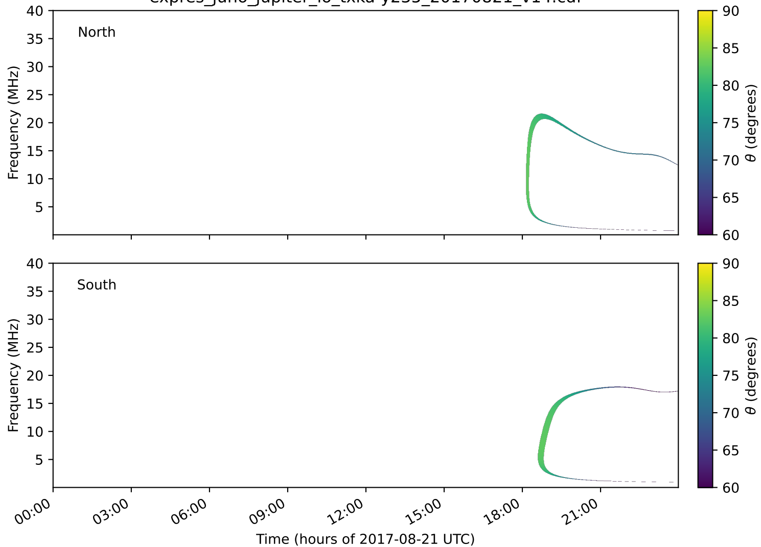
expres_juno_jupiter_io_txka-y235_20170821_v14.cdf
