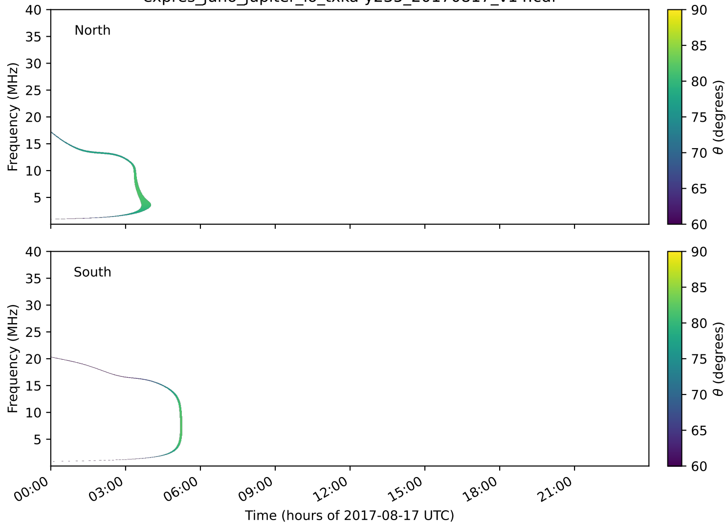
expres_juno_jupiter_io_txka-y235_20170817_v14.cdf
