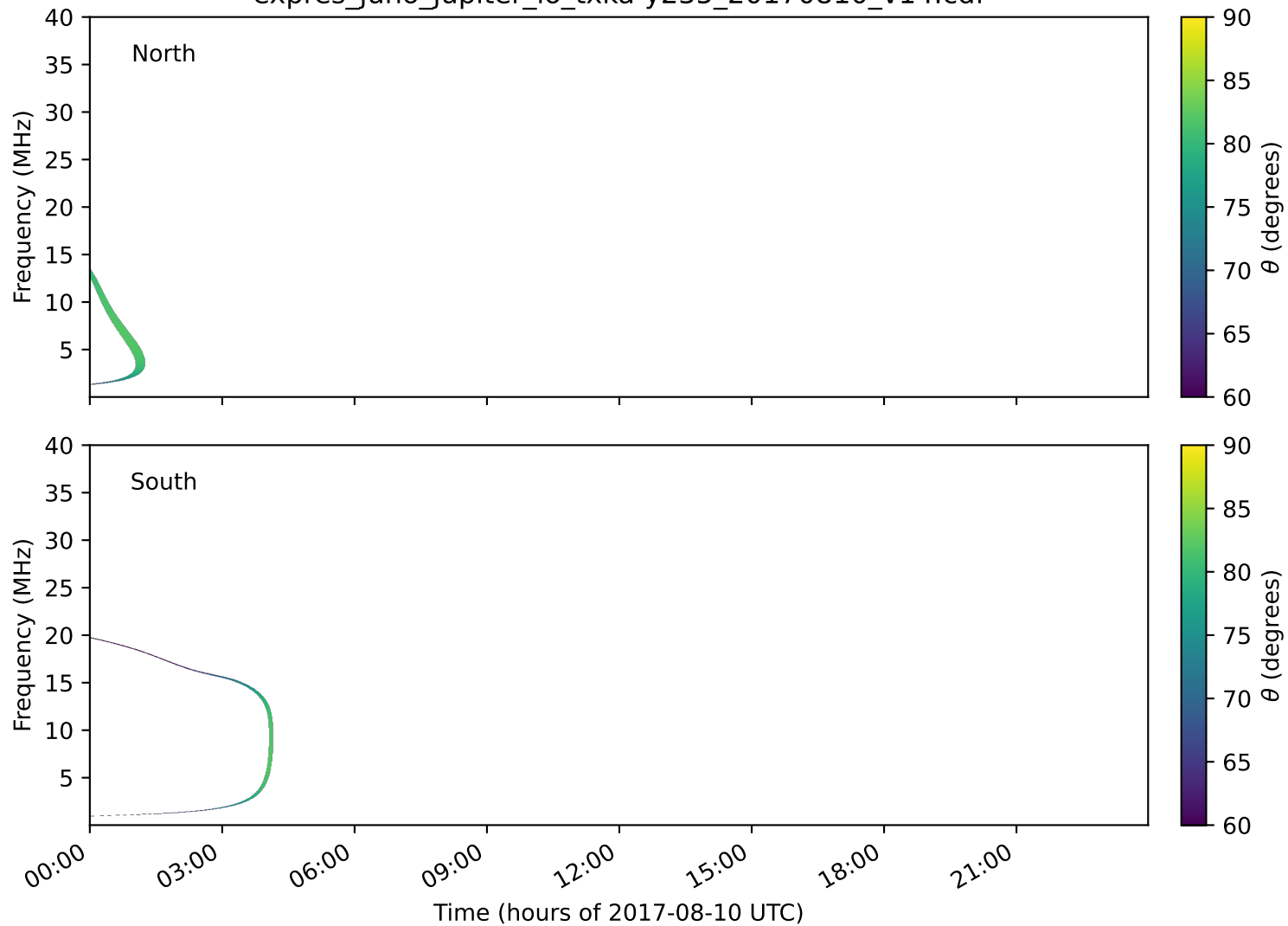
expres_juno_jupiter_io_txka-y235_20170810_v14.cdf
