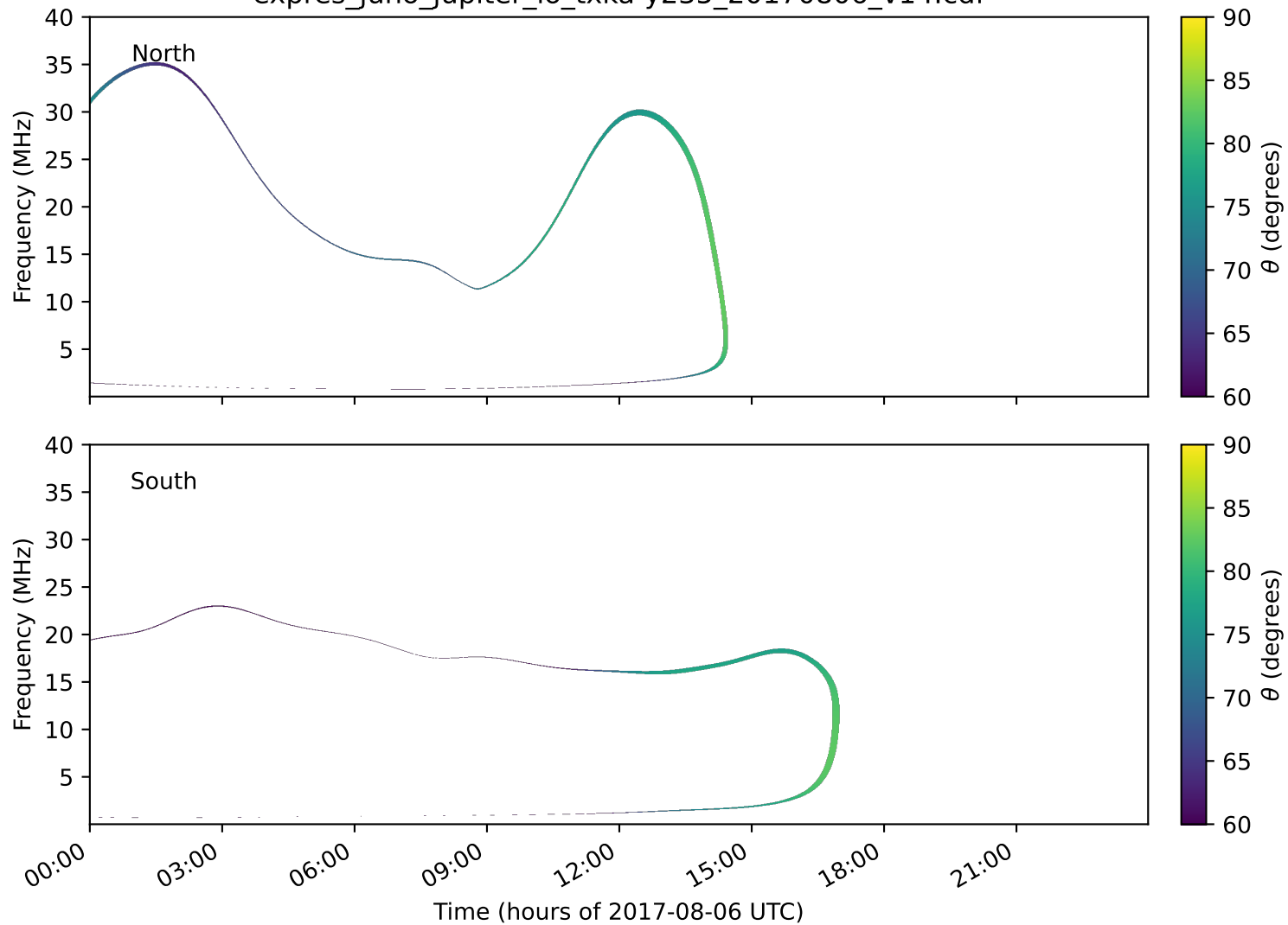
expres_juno_jupiter_io_txka-y235_20170806_v14.cdf
