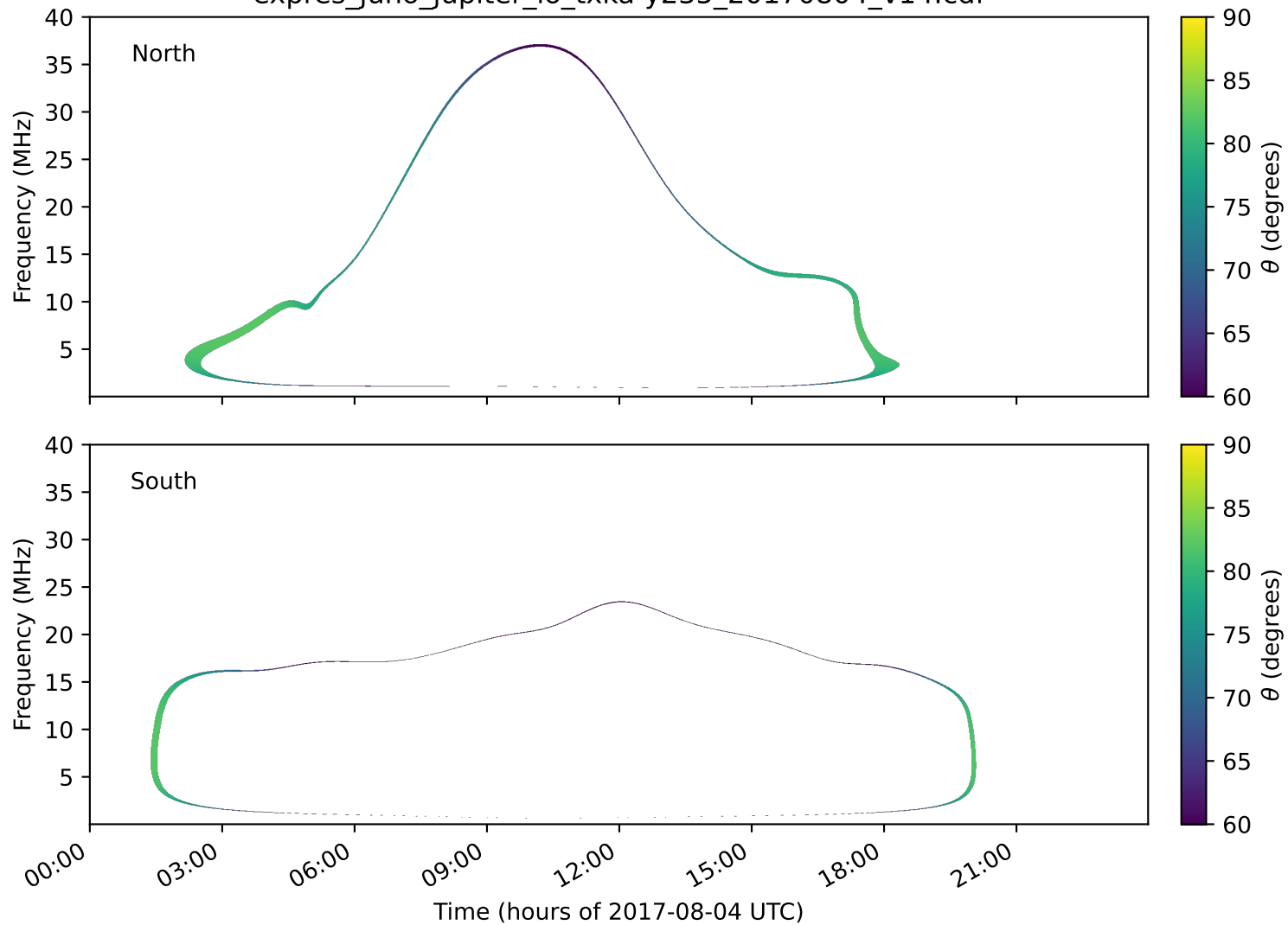
expres_juno_jupiter_io_txka-y235_20170804_v14.cdf
