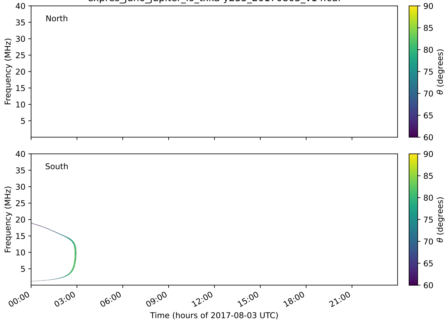
expres_juno_jupiter_io_txka-y235_20170803_v14.cdf
