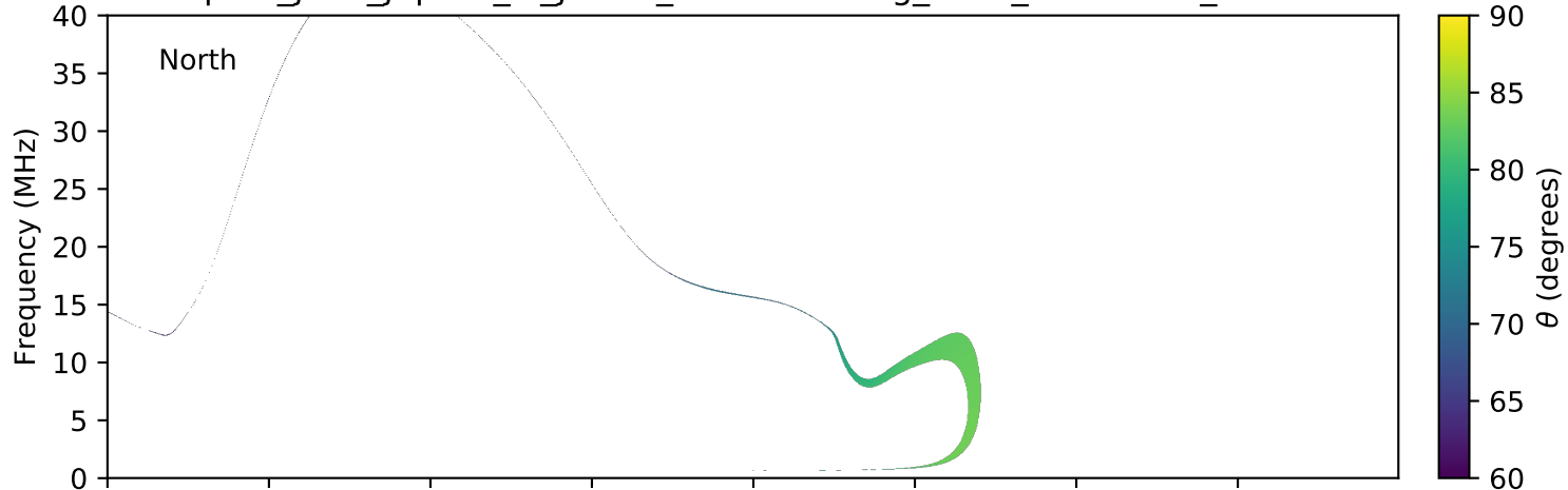
expres_juno_jupiter_io_jrm09_lossc-wid1deg_3kev_20170829_v01.cdf
