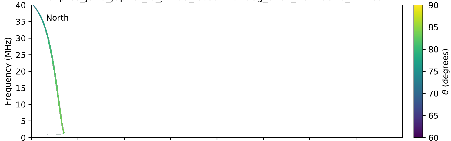
expres_juno_jupiter_io_jrm09_lossc-wid1deg_3kev_20170826_v01.cdf
