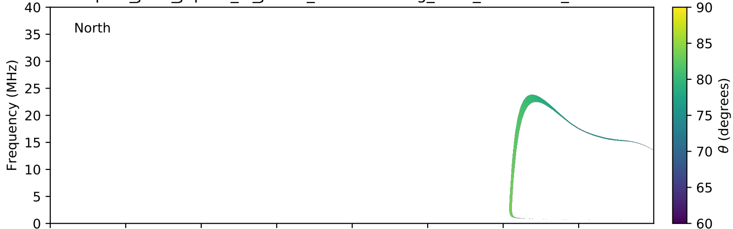
expres_juno_jupiter_io_jrm09_lossc-wid1deg_3kev_20170821_v01.cdf
