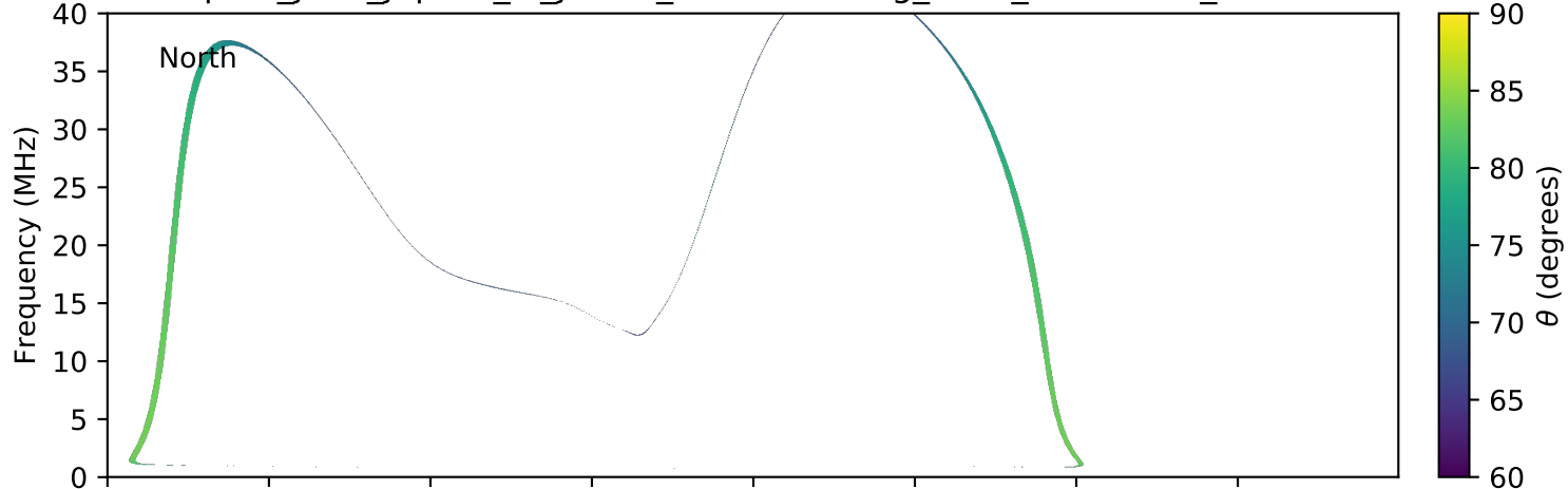
expres_juno_jupiter_io_jrm09_lossc-wid1deg_3kev_20170820_v01.cdf
