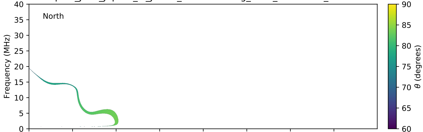
expres_juno_jupiter_io_jrm09_lossc-wid1deg_3kev_20170817_v01.cdf
