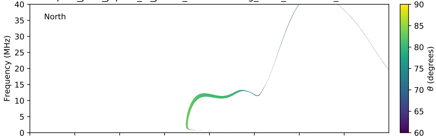
expres_juno_jupiter_io_jrm09_lossc-wid1deg_3kev_20170816_v01.cdf
