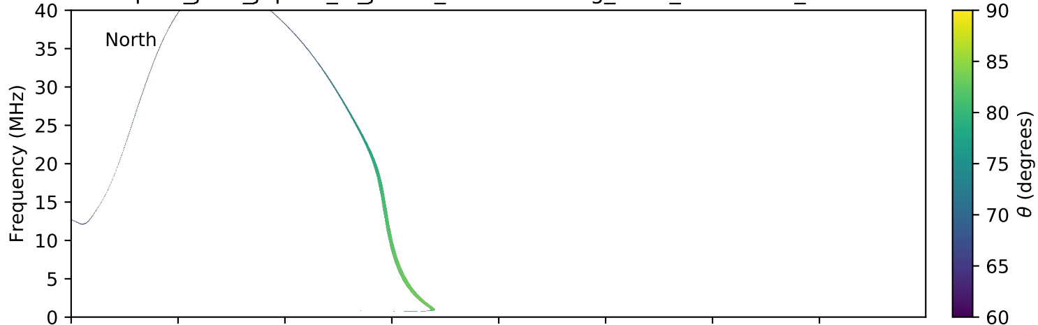
expres_juno_jupiter_io_jrm09_lossc-wid1deg_3kev_20170815_v01.cdf
