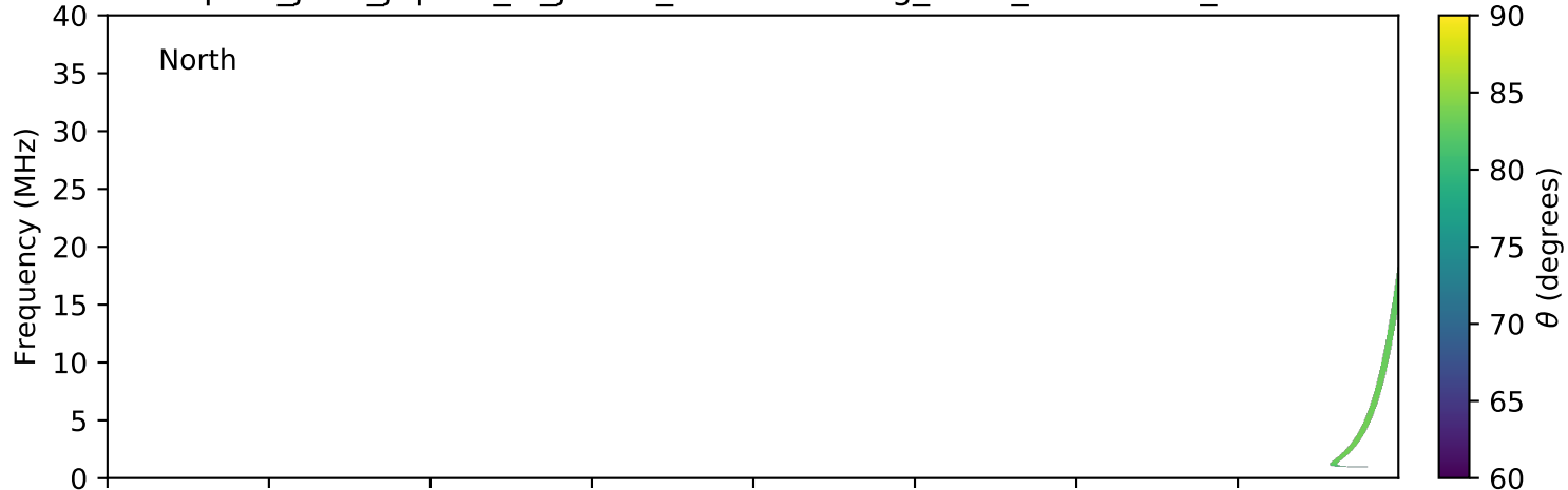
expres_juno_jupiter_io_jrm09_lossc-wid1deg_3kev_20170812_v01.cdf
