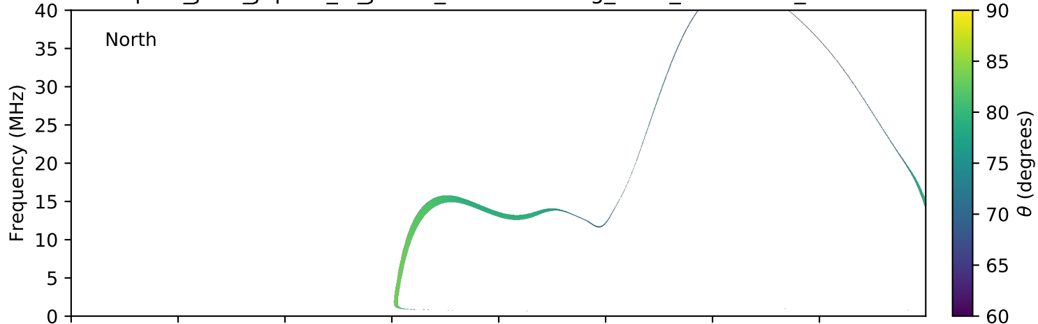
expres_juno_jupiter_io_jrm09_lossc-wid1deg_3kev_20170809_v01.cdf
