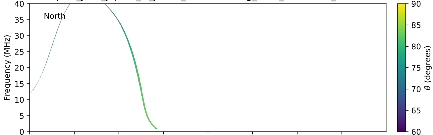
expres_juno_jupiter_io_jrm09_lossc-wid1deg_3kev_20170808_v01.cdf
