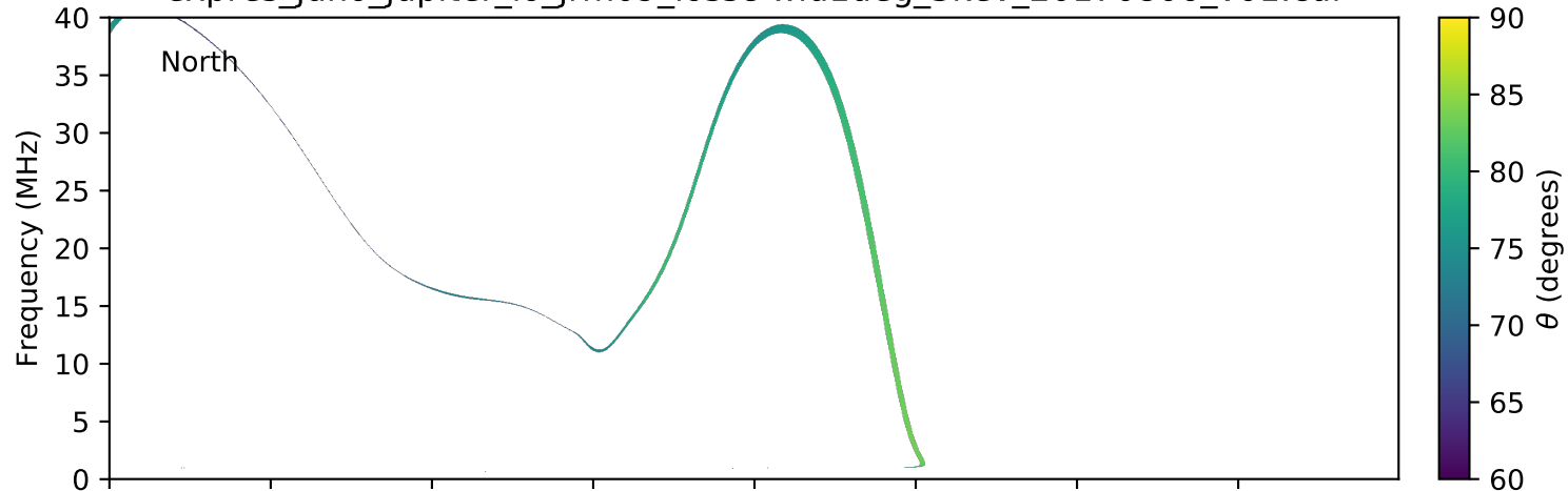
expres_juno_jupiter_io_jrm09_lossc-wid1deg_3kev_20170806_v01.cdf
