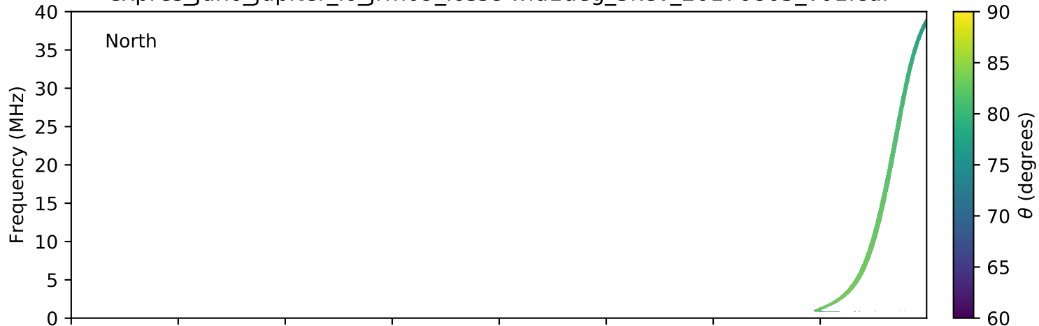
expres_juno_jupiter_io_jrm09_lossc-wid1deg_3kev_20170805_v01.cdf
