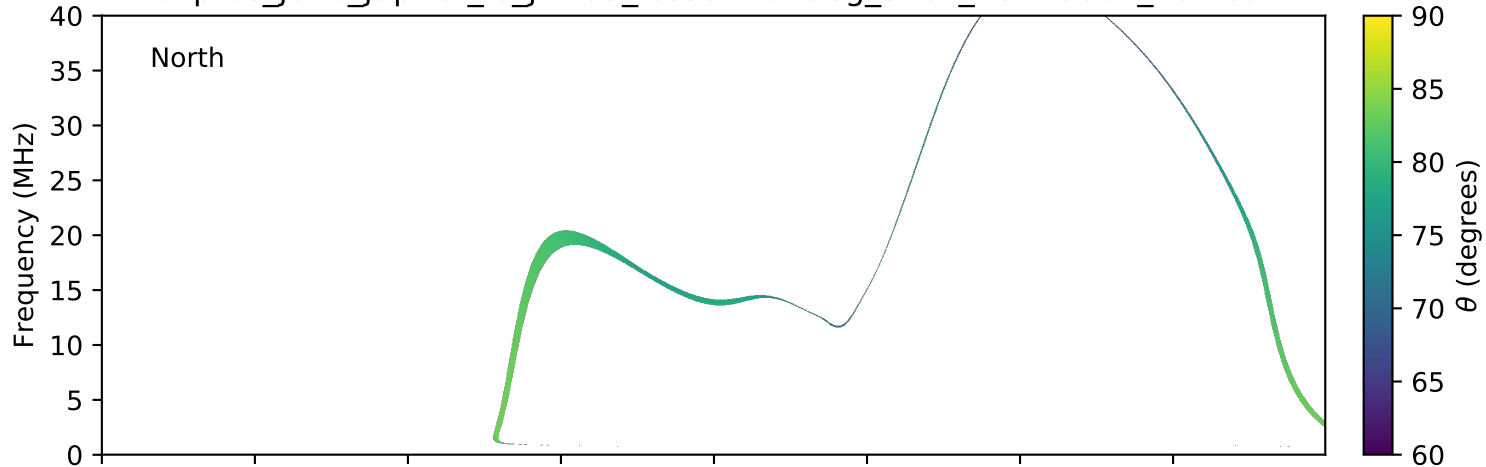
expres_juno_jupiter_io_jrm09_lossc-wid1deg_3kev_20170802_v01.cdf
