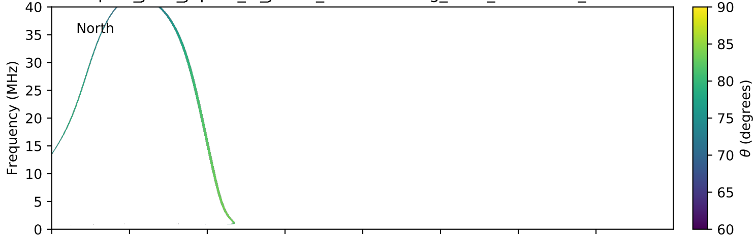
expres_juno_jupiter_io_jrm09_lossc-wid1deg_3kev_20170801_v01.cdf
