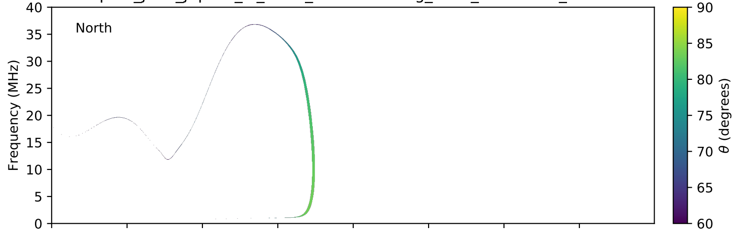
expres_juno_jupiter_io_isaac_lossc-wid1deg_3kev_20170831_v01.cdf
