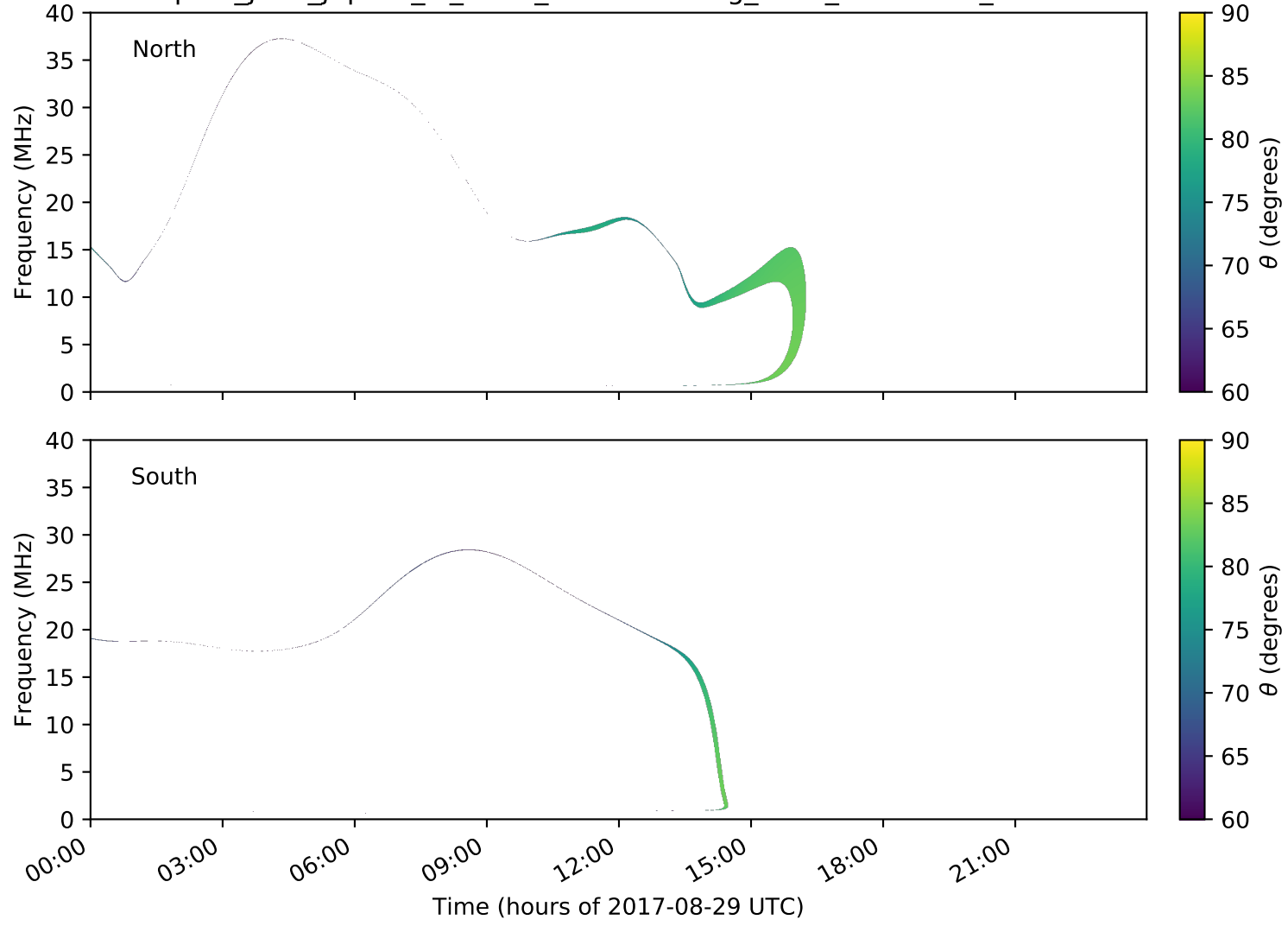
expres_juno_jupiter_io_isaac_lossc-wid1deg_3kev_20170829_v01.cdf
