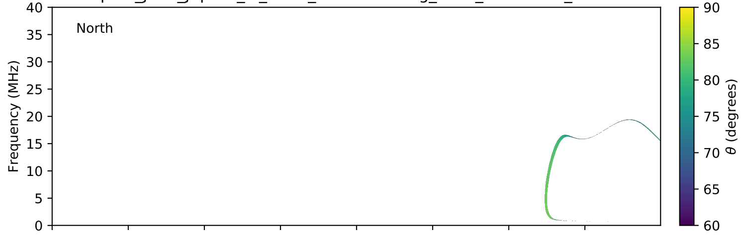
expres_juno_jupiter_io_isaac_lossc-wid1deg_3kev_20170828_v01.cdf
