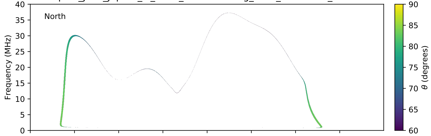
expres_juno_jupiter_io_isaac_lossc-wid1deg_3kev_20170827_v01.cdf
