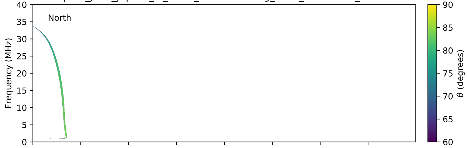
expres_juno_jupiter_io_isaac_lossc-wid1deg_3kev_20170826_v01.cdf
