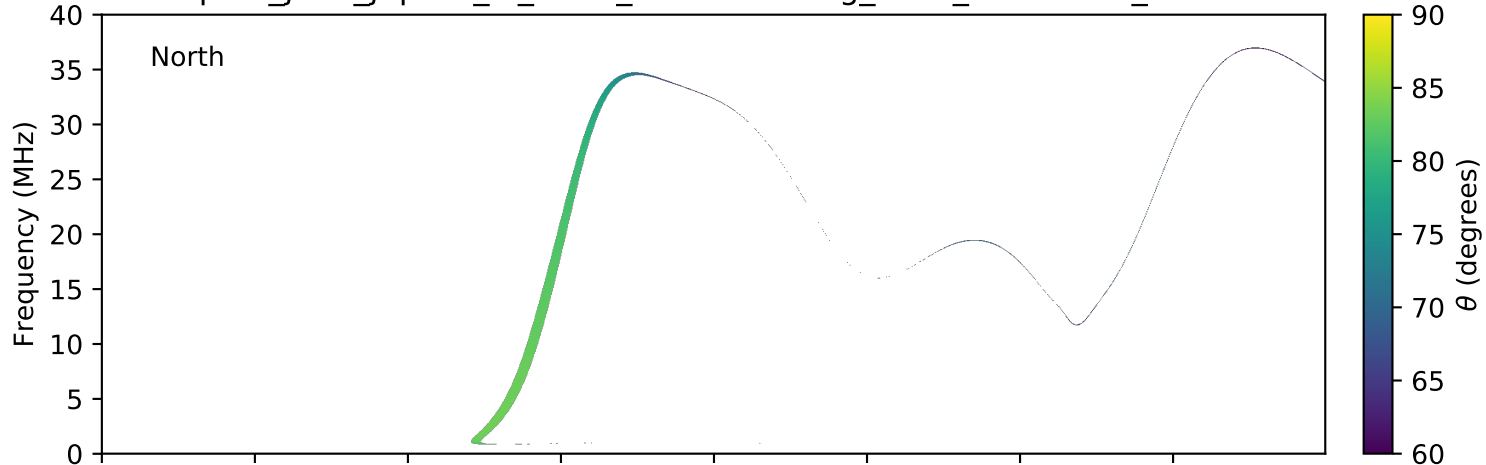
expres_juno_jupiter_io_isaac_lossc-wid1deg_3kev_20170825_v01.cdf
