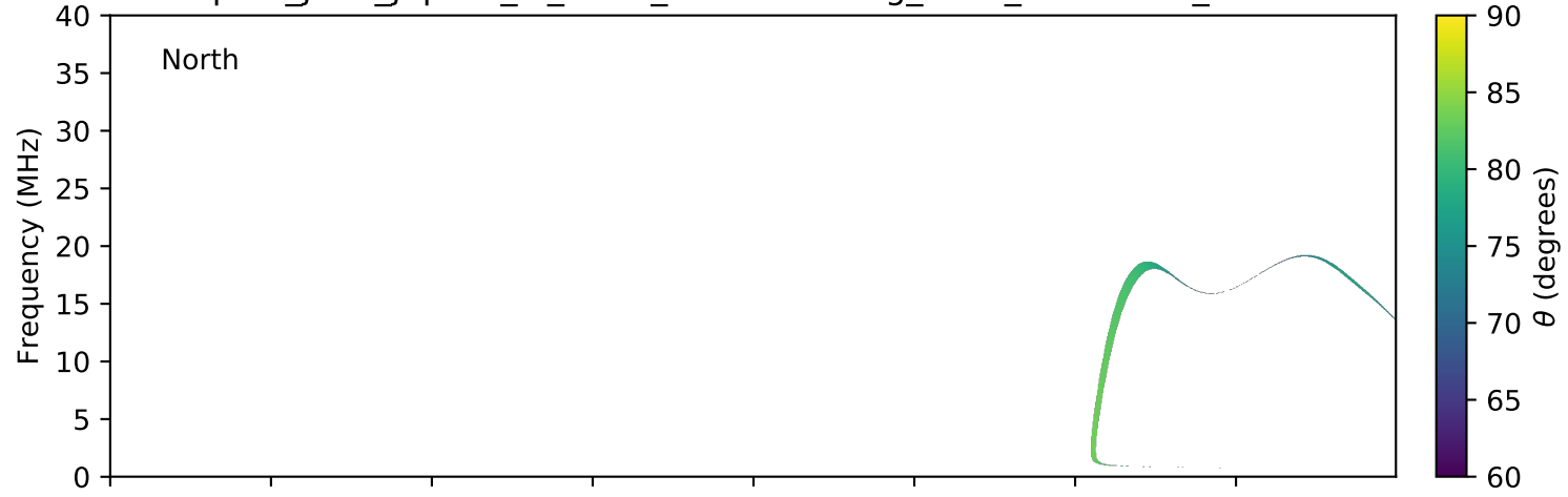
expres_juno_jupiter_io_isaac_lossc-wid1deg_3kev_20170821_v01.cdf
