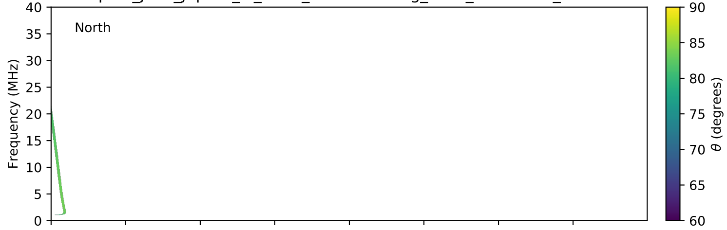
expres_juno_jupiter_io_isaac_lossc-wid1deg_3kev_20170819_v01.cdf
