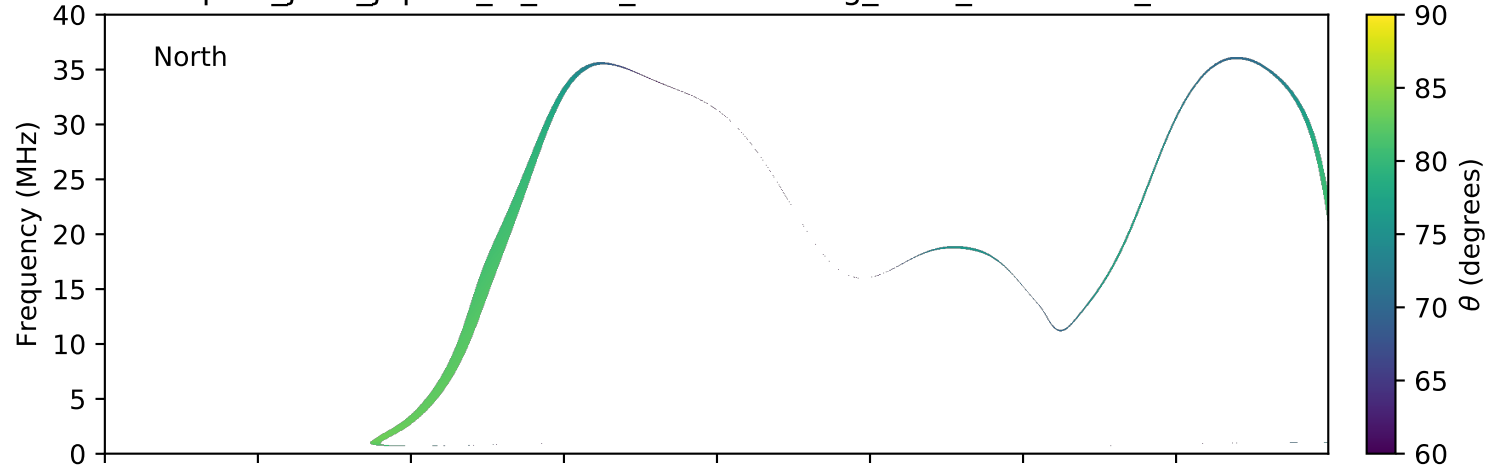
expres_juno_jupiter_io_isaac_lossc-wid1deg_3kev_20170818_v01.cdf
