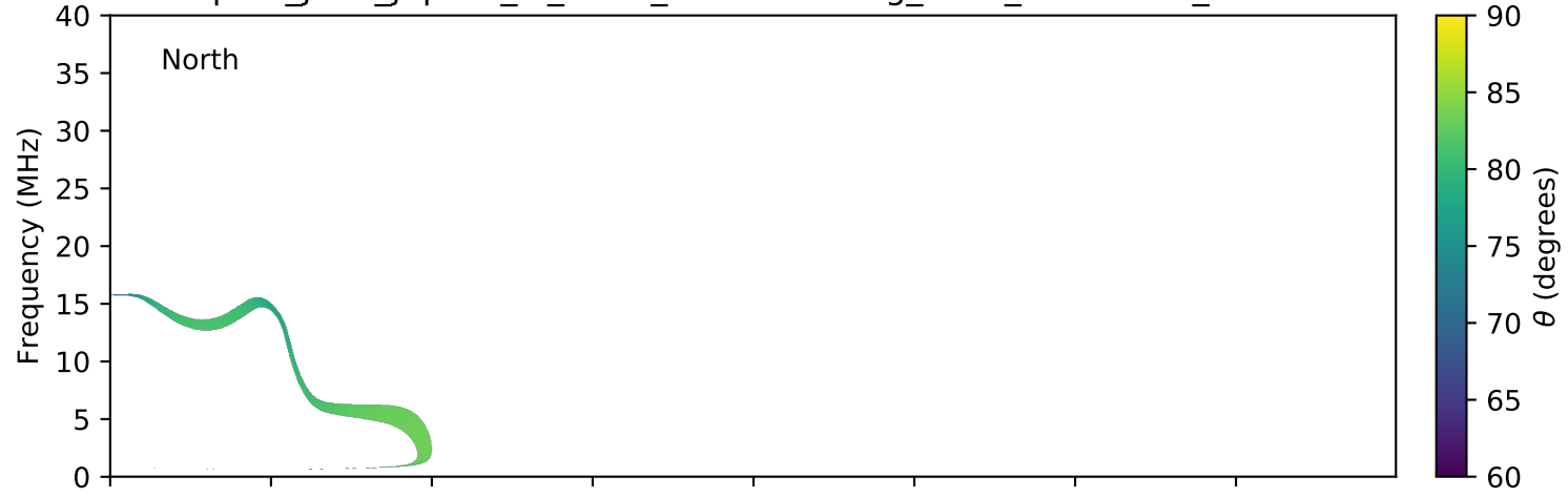
expres_juno_jupiter_io_isaac_lossc-wid1deg_3kev_20170817_v01.cdf
