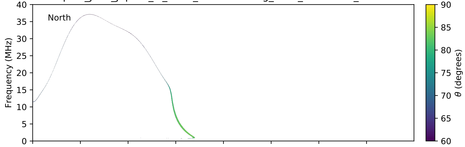
expres_juno_jupiter_io_isaac_lossc-wid1deg_3kev_20170815_v01.cdf
