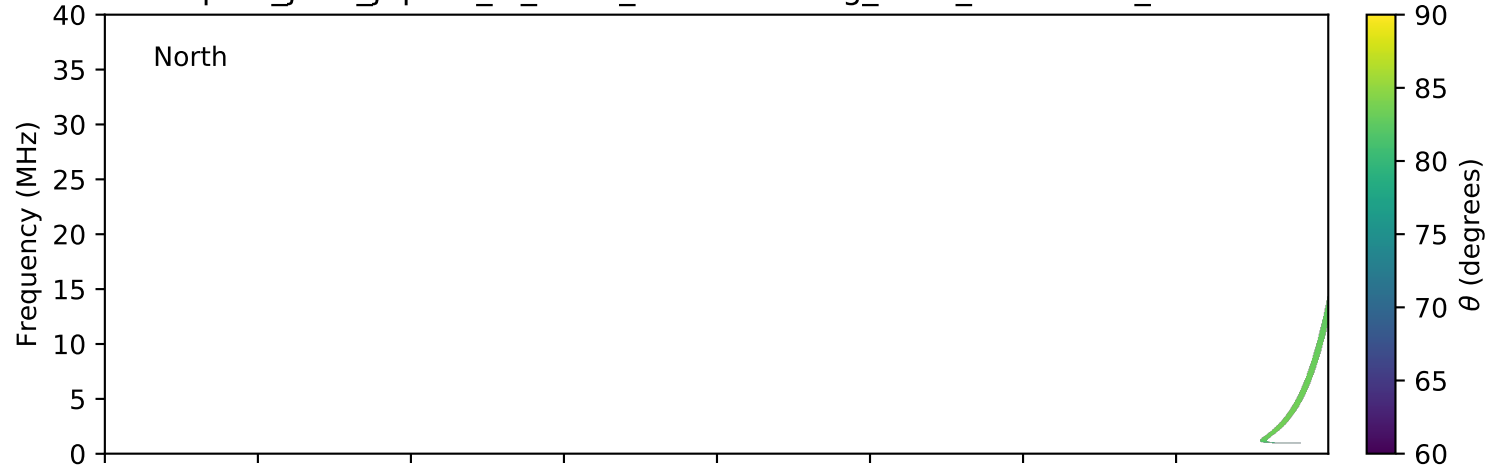
expres_juno_jupiter_io_isaac_lossc-wid1deg_3kev_20170812_v01.cdf
