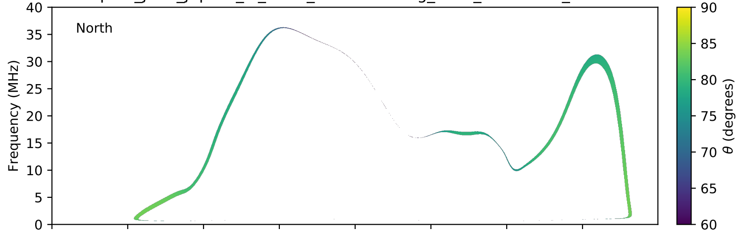
expres_juno_jupiter_io_isaac_lossc-wid1deg_3kev_20170811_v01.cdf
