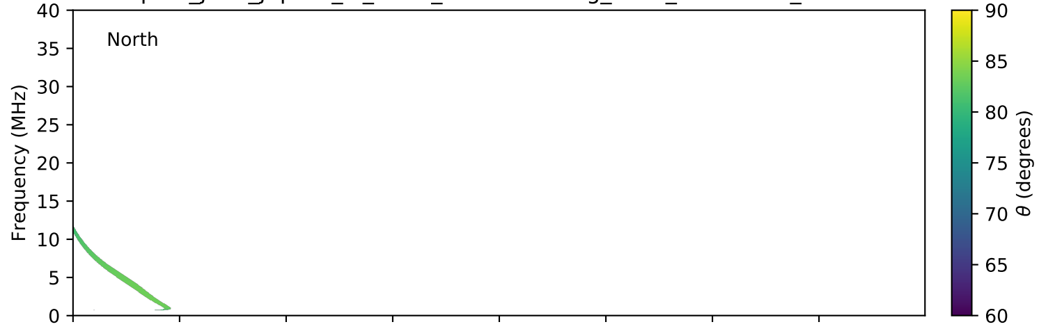
expres_juno_jupiter_io_isaac_lossc-wid1deg_3kev_20170810_v01.cdf
