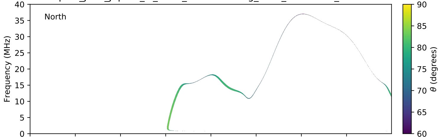
expres_juno_jupiter_io_isaac_lossc-wid1deg_3kev_20170809_v01.cdf
