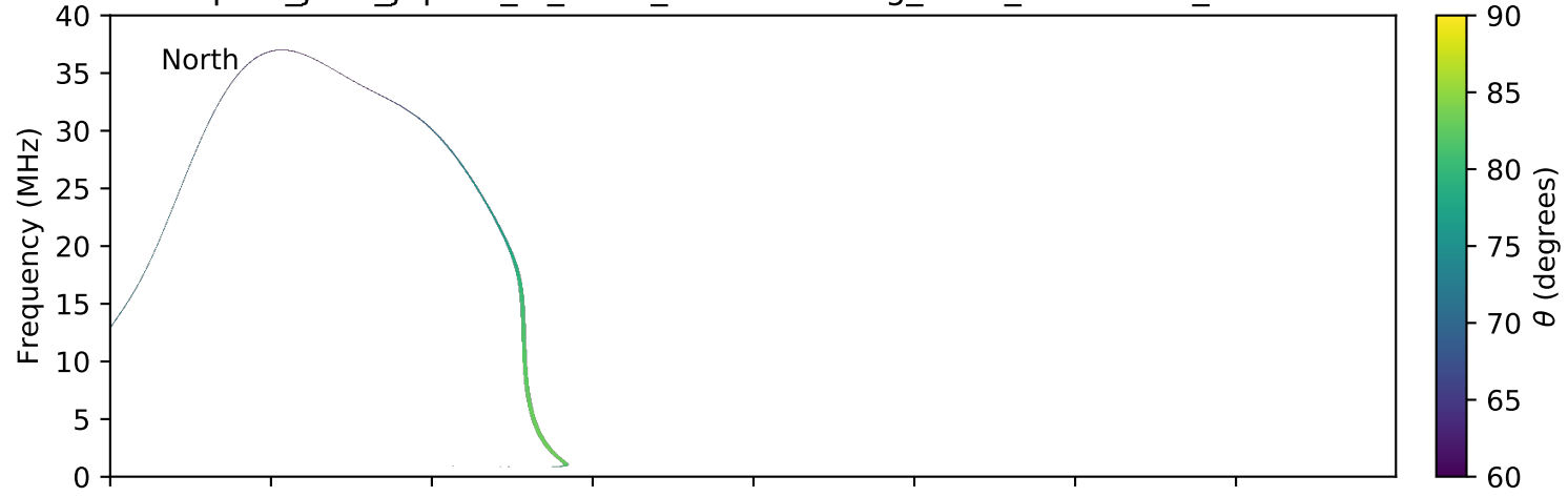
expres_juno_jupiter_io_isaac_lossc-wid1deg_3kev_20170808_v01.cdf
