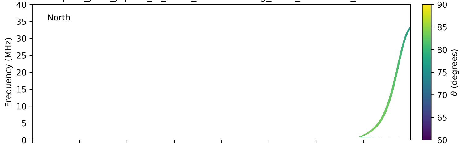
expres_juno_jupiter_io_isaac_lossc-wid1deg_3kev_20170805_v01.cdf
