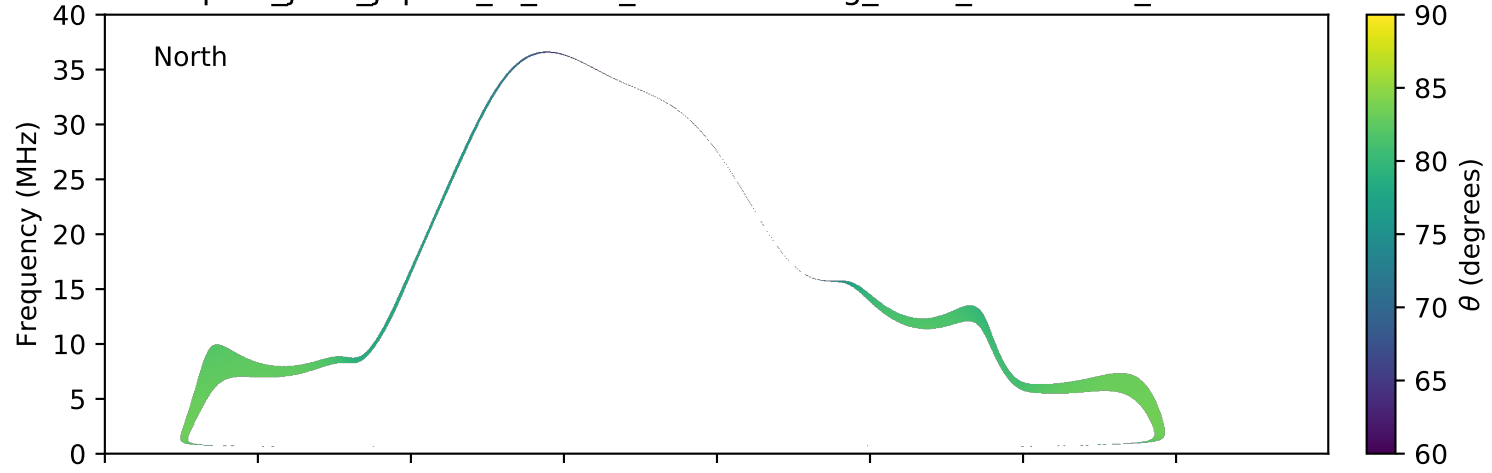
expres_juno_jupiter_io_isaac_lossc-wid1deg_3kev_20170804_v01.cdf
