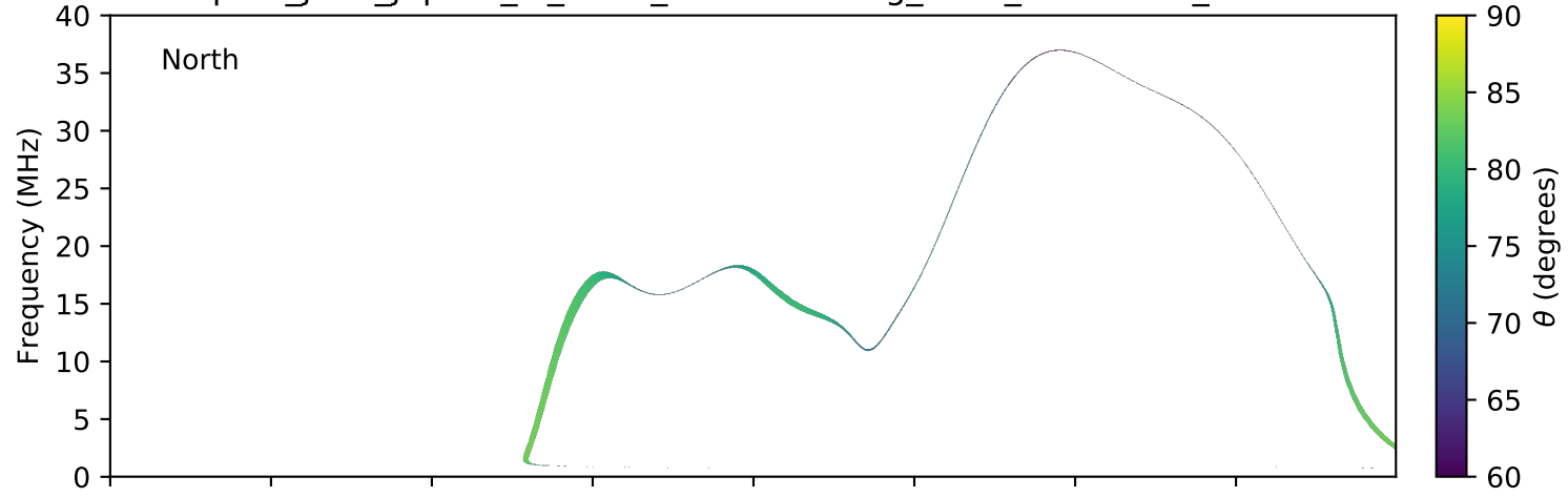
expres_juno_jupiter_io_isaac_lossc-wid1deg_3kev_20170802_v01.cdf
