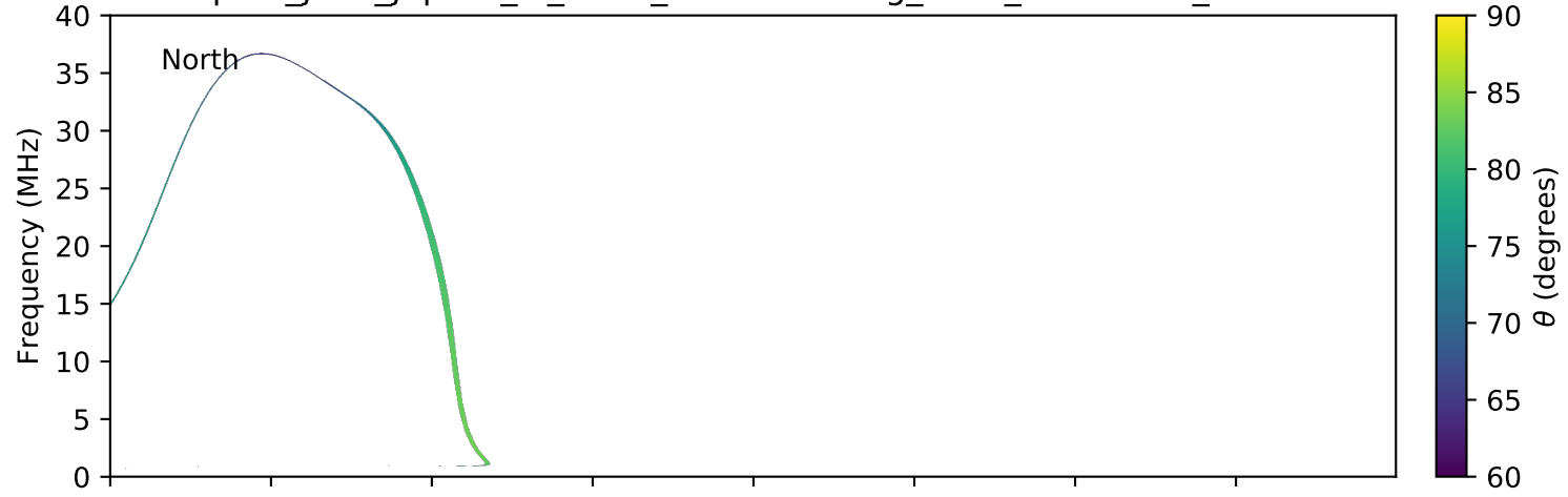
expres_juno_jupiter_io_isaac_lossc-wid1deg_3kev_20170801_v01.cdf
