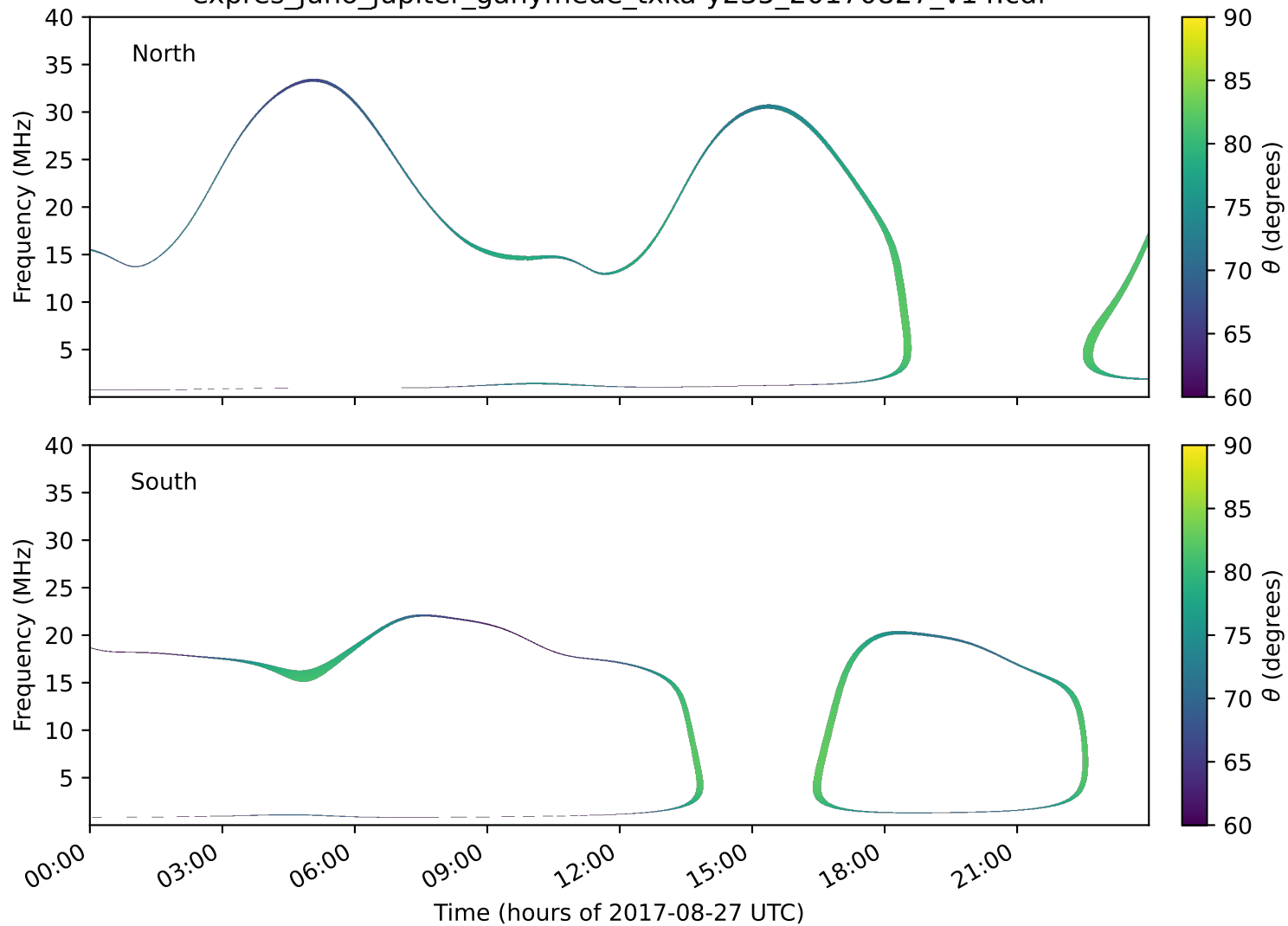
expres_juno_jupiter_ganymede_txka-y235_20170827_v14.cdf
