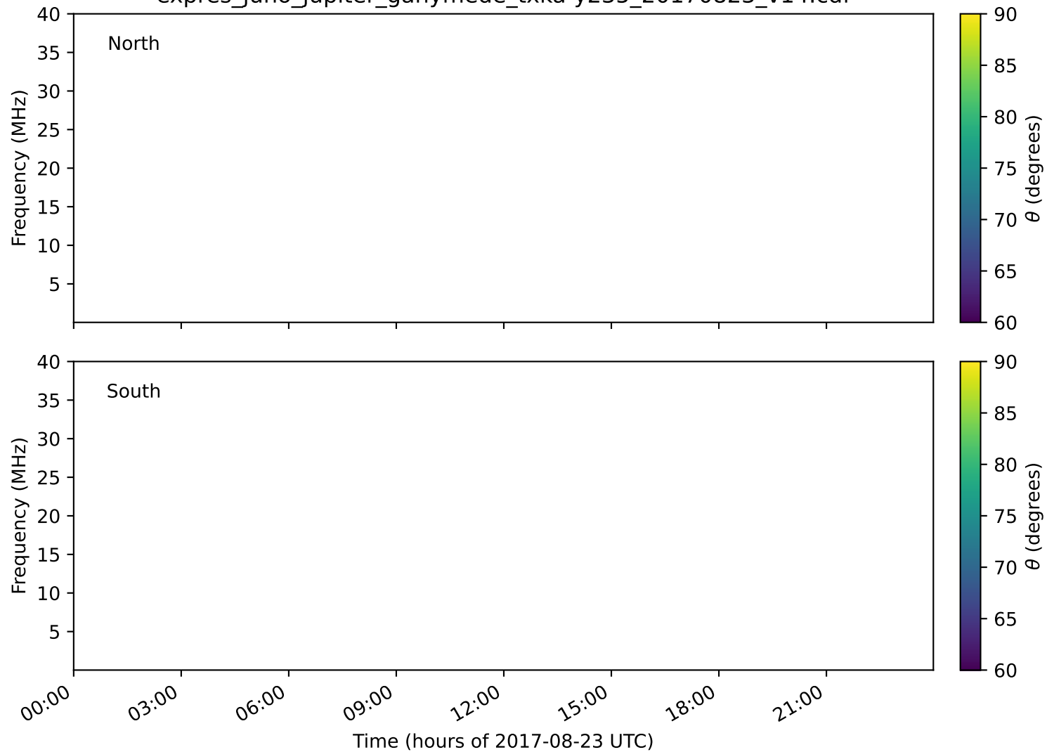
expres_juno_jupiter_ganymede_txka-y235_20170823_v14.cdf
