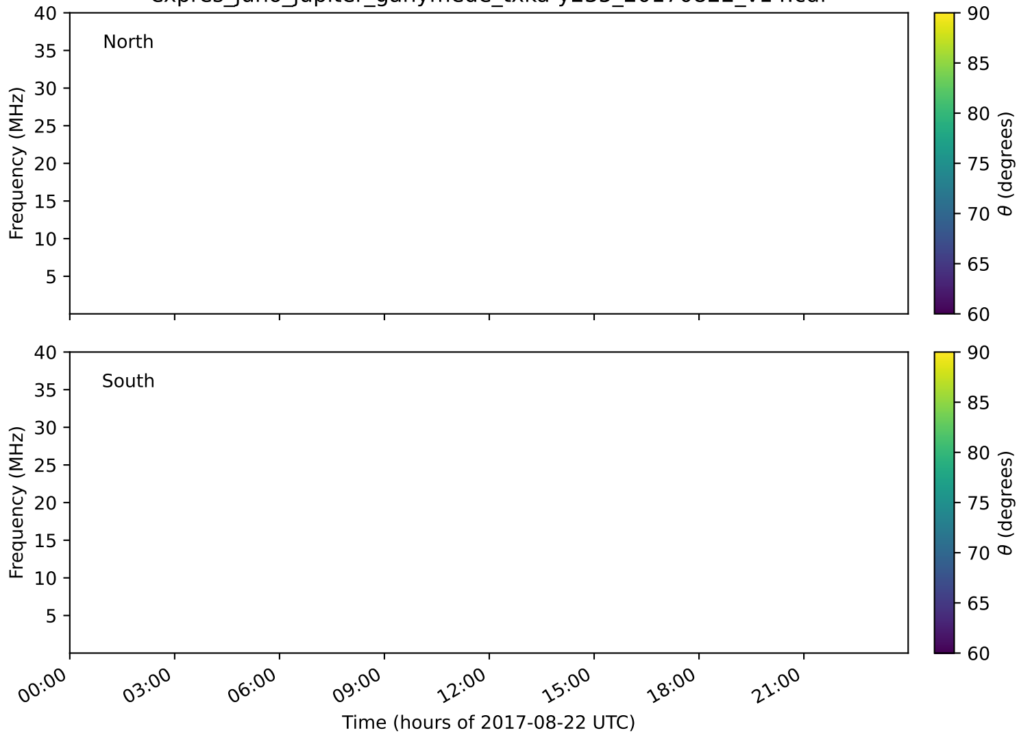
expres_juno_jupiter_ganymede_txka-y235_20170822_v14.cdf
