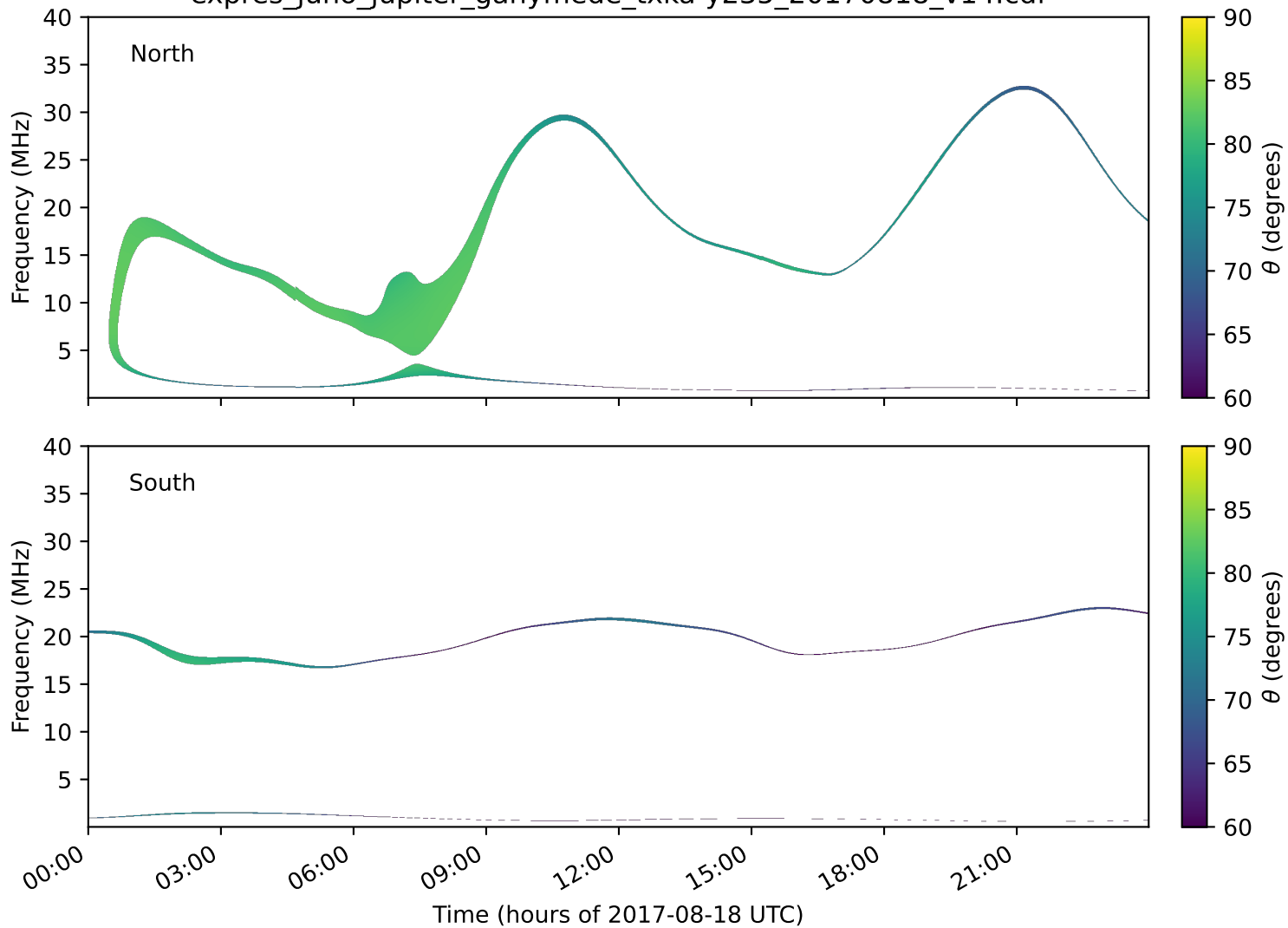
expres_juno_jupiter_ganymede_txka-y235_20170818_v14.cdf
