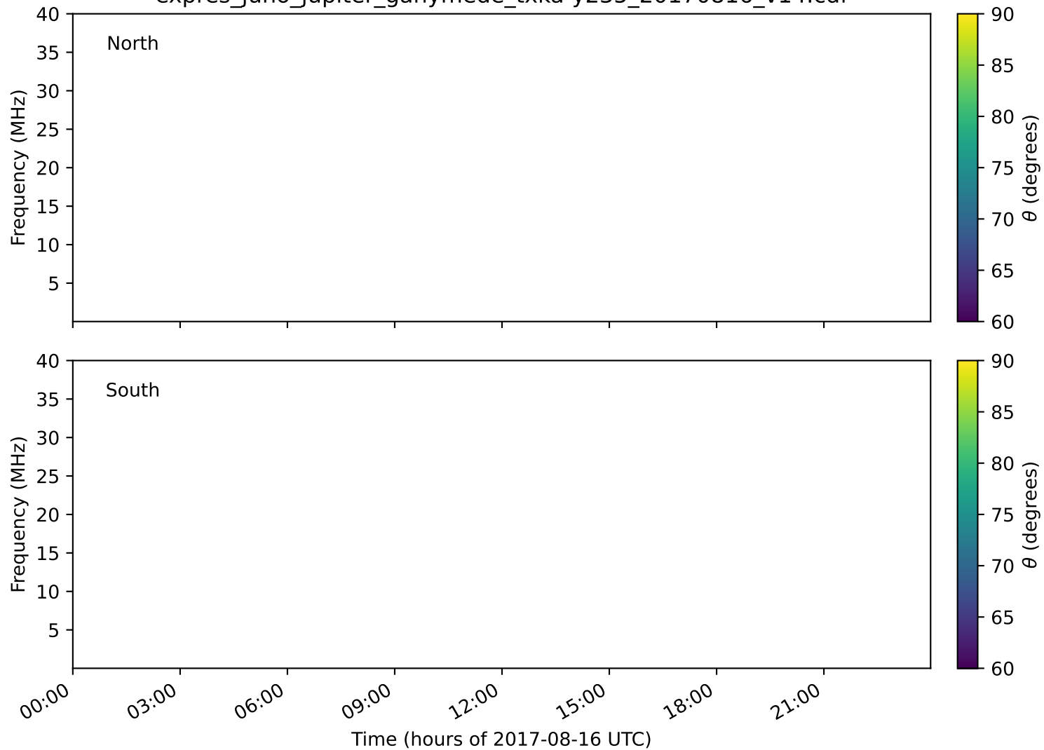
expres_juno_jupiter_ganymede_txka-y235_20170816_v14.cdf
