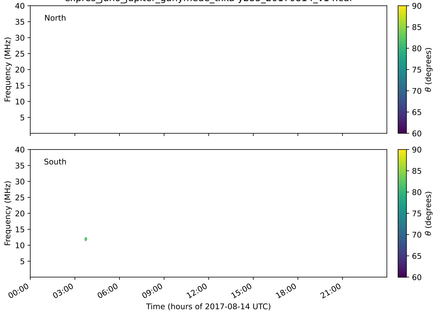
expres_juno_jupiter_ganymede_txka-y235_20170814_v14.cdf
